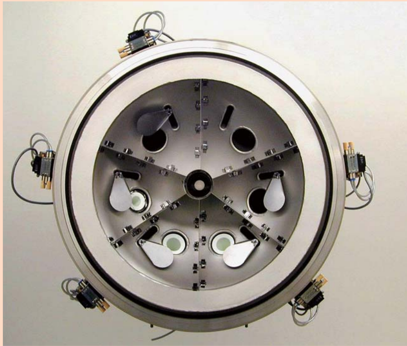
UHV flange for Effusion Cells with LN 2 shroud
